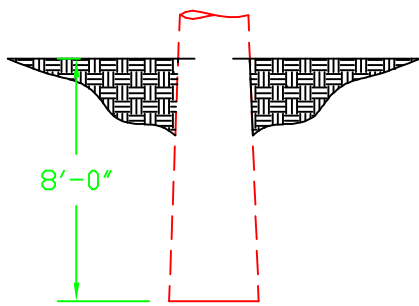
60' Structure Embedment
