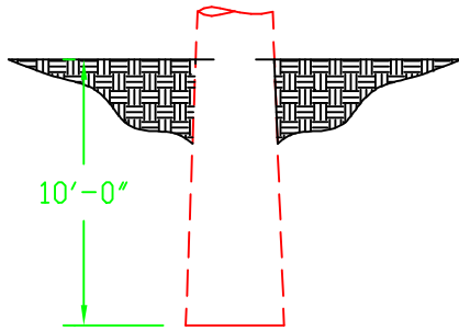
80' Structure Embedment
