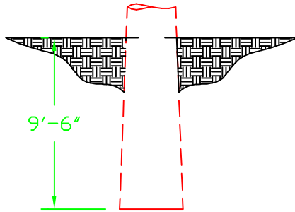
75' Structure Embedment
