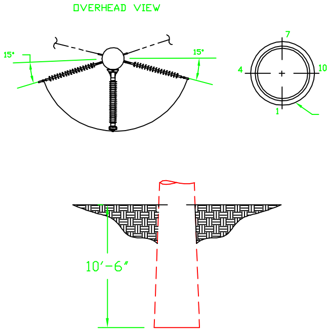
85' Structure Embedment
